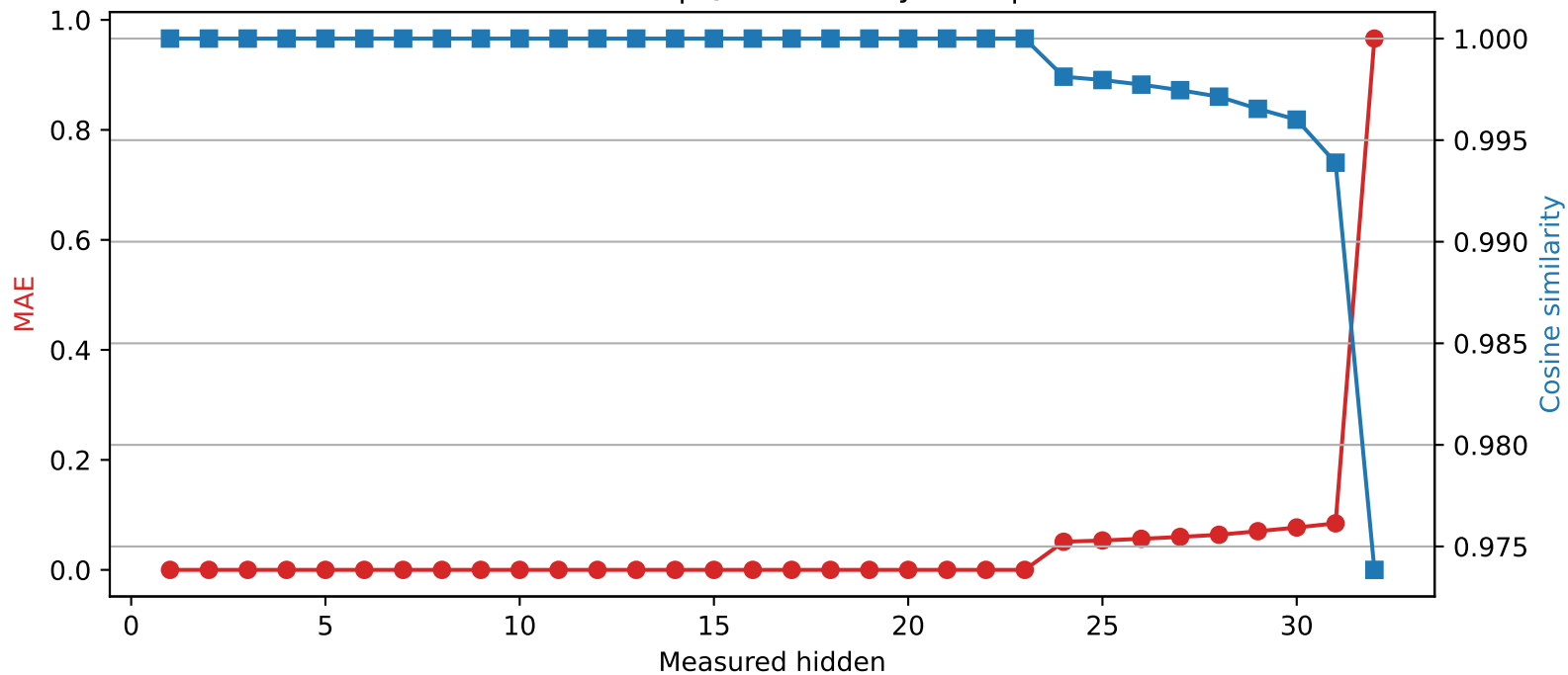
Mistral-7B-Instruct-v0.3 | Quantized layer 23 | float16 → int4
