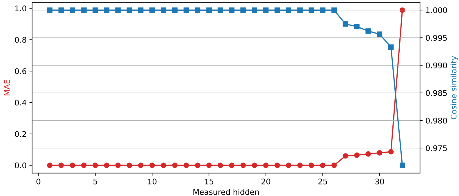
Mistral-7B-Instruct-v0.3 | Quantized layer 26 | float16 → int4
