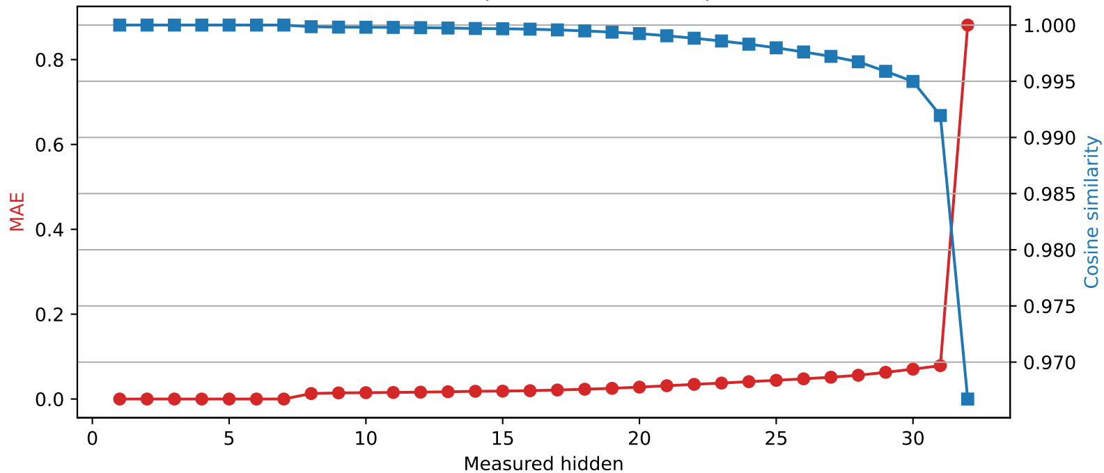
Mistral-7B-Instruct-v0.3 | Quantized layer 7 | float16 → int4
