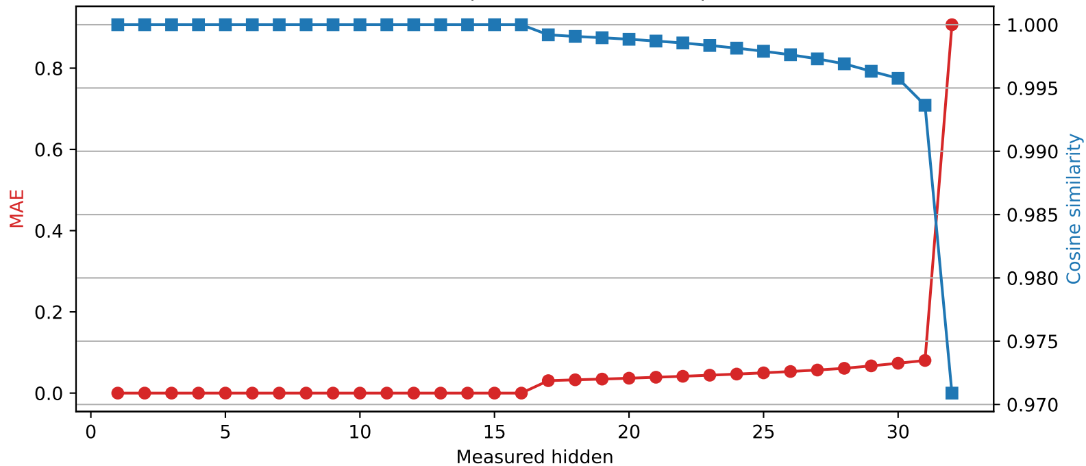
Mistral-7B-Instruct-v0.3 | Quantized layer 16 | float16 → int4
