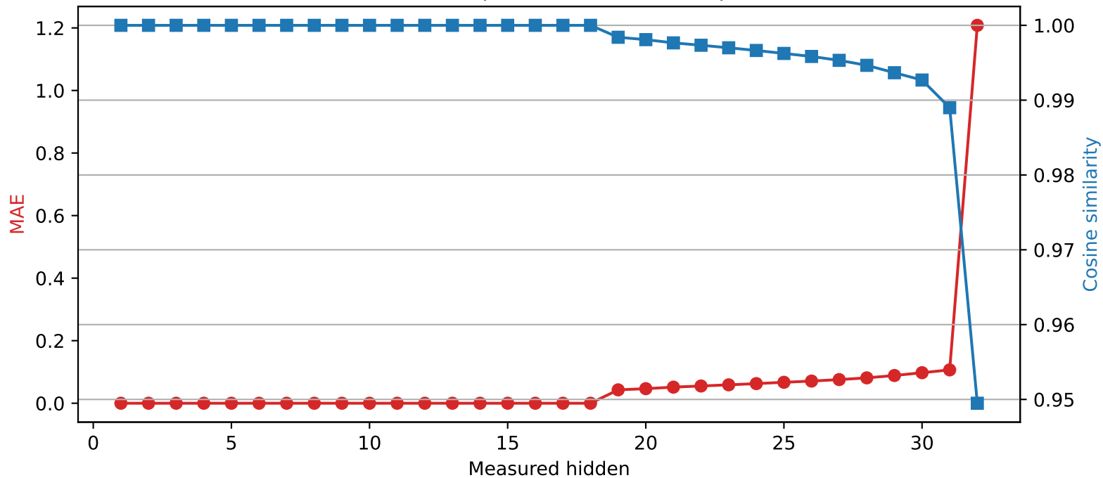
Mistral-7B-Instruct-v0.3 | Quantized layer 18 | float16 \rightarrow int4
