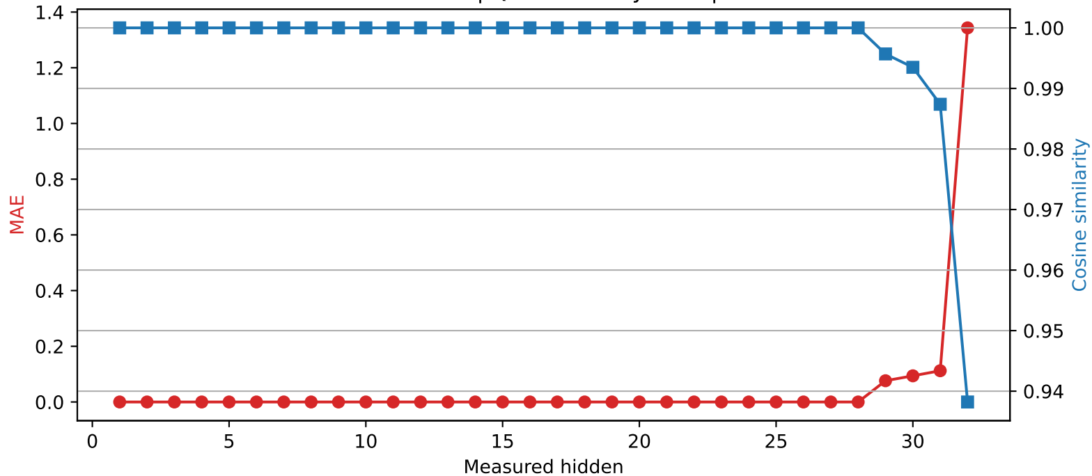
Mistral-7B-Instruct-v0.3 | Quantized layer 28 | float16 \rightarrow int4
