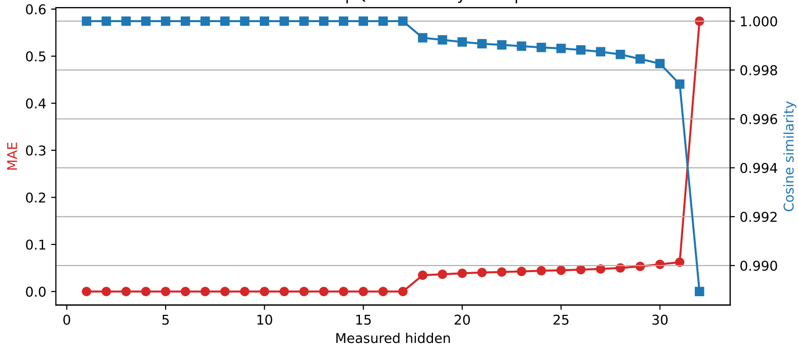
Mistral-7B-Instruct-v0.3 | Quantized layer 17 | float16 → int4
