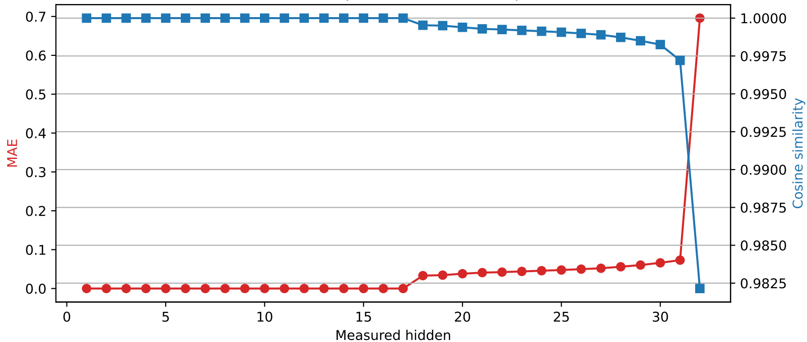
Mistral-7B-Instruct-v0.3 | Quantized layer 17 | float32 → int4
