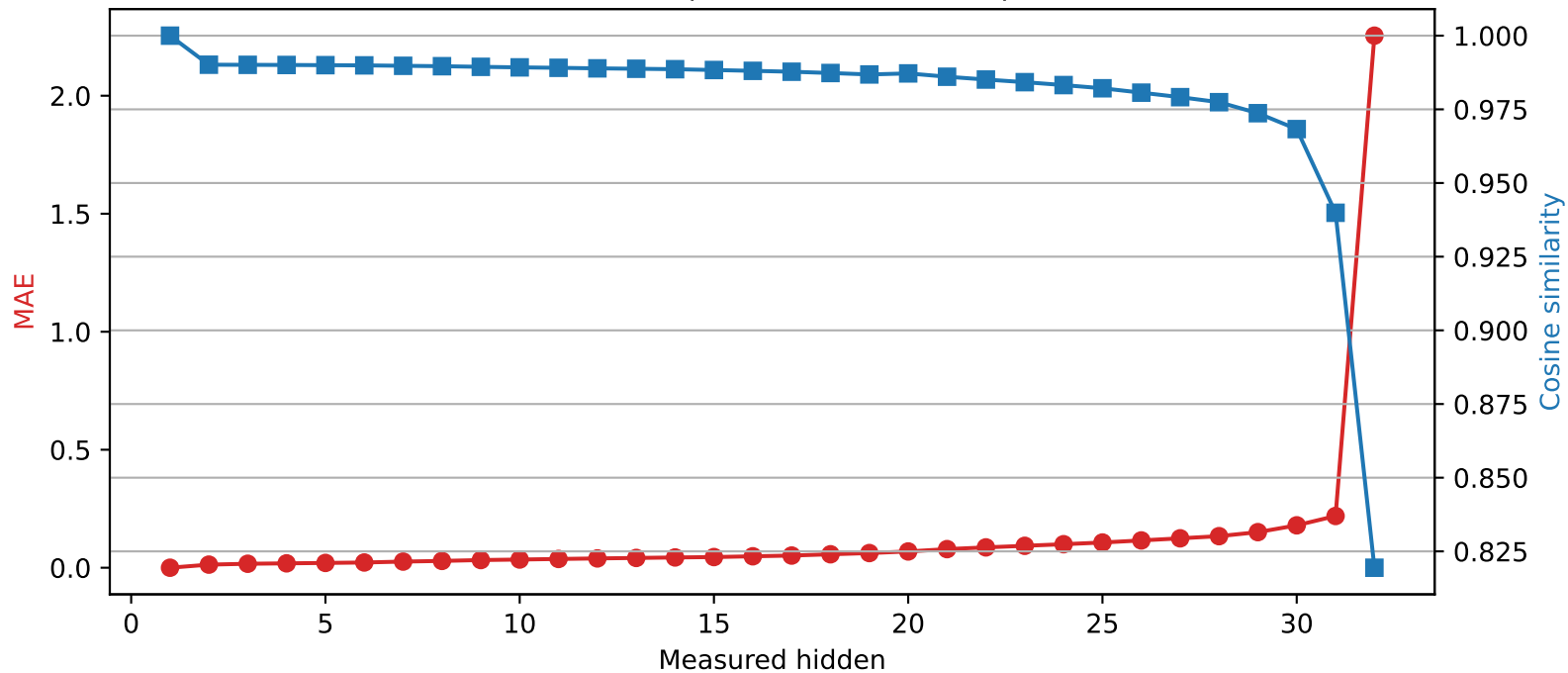
Mistral-7B-Instruct-v0.3 | Quantized layer 1 | float32 → int4
