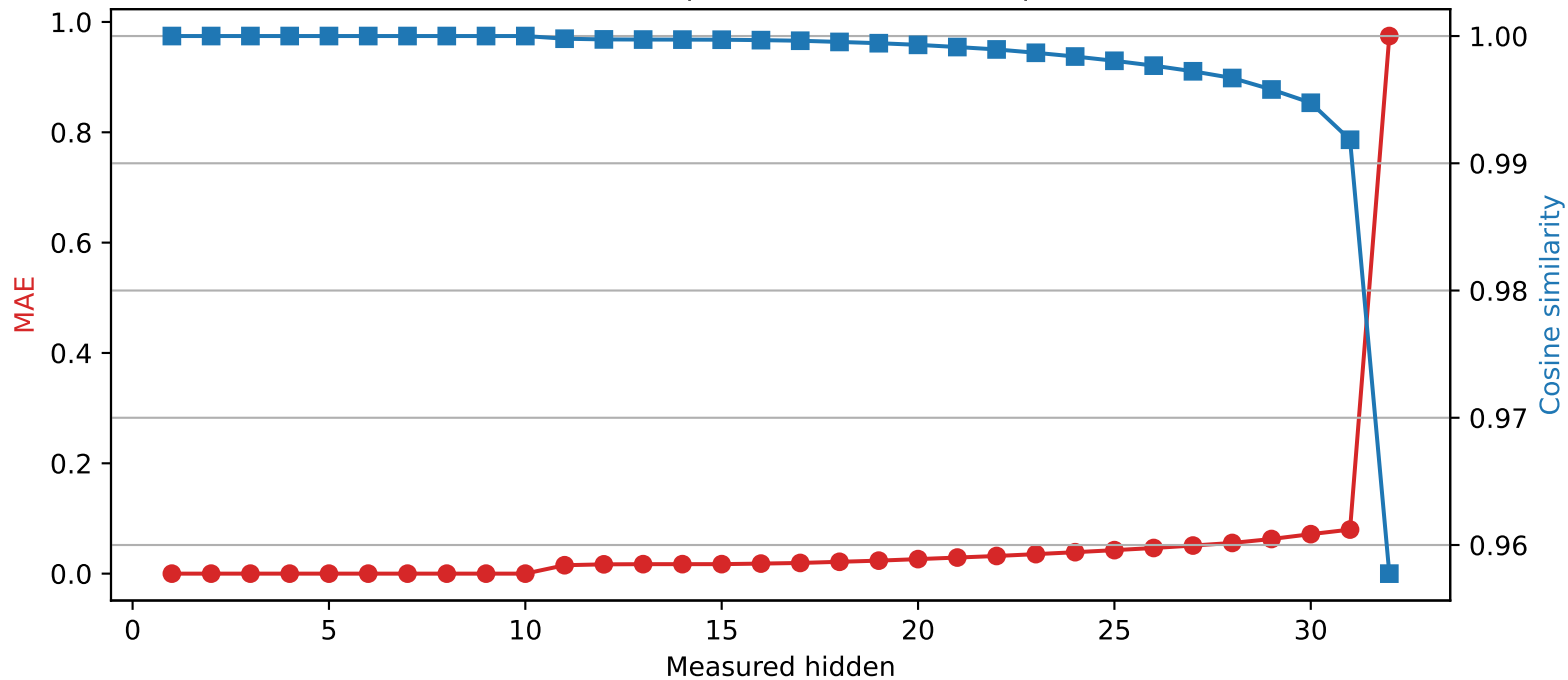
Mistral-7B-Instruct-v0.3 | Quantized layer 10 | float32 → int4
