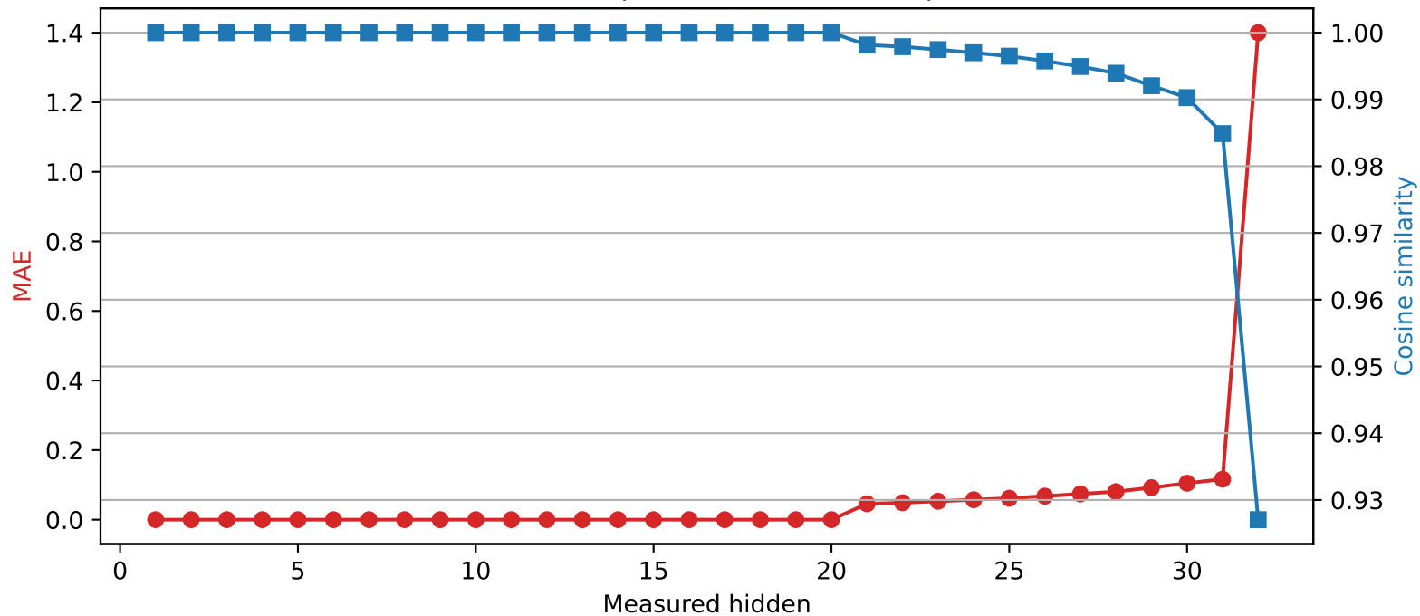
Mistral-7B-Instruct-v0.3 | Quantized layer 20 | float32 → int4
