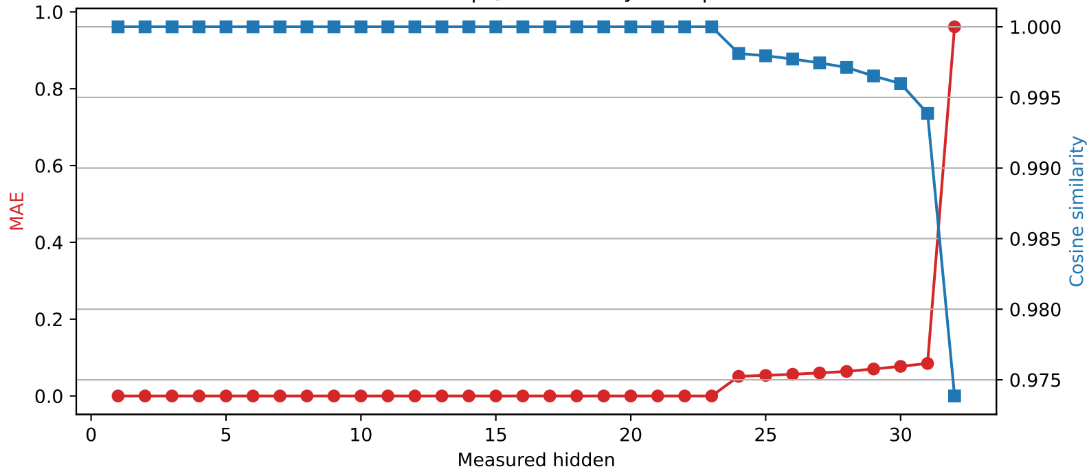
Mistral-7B-Instruct-v0.3 | Quantized layer 23 | float32 → int4
