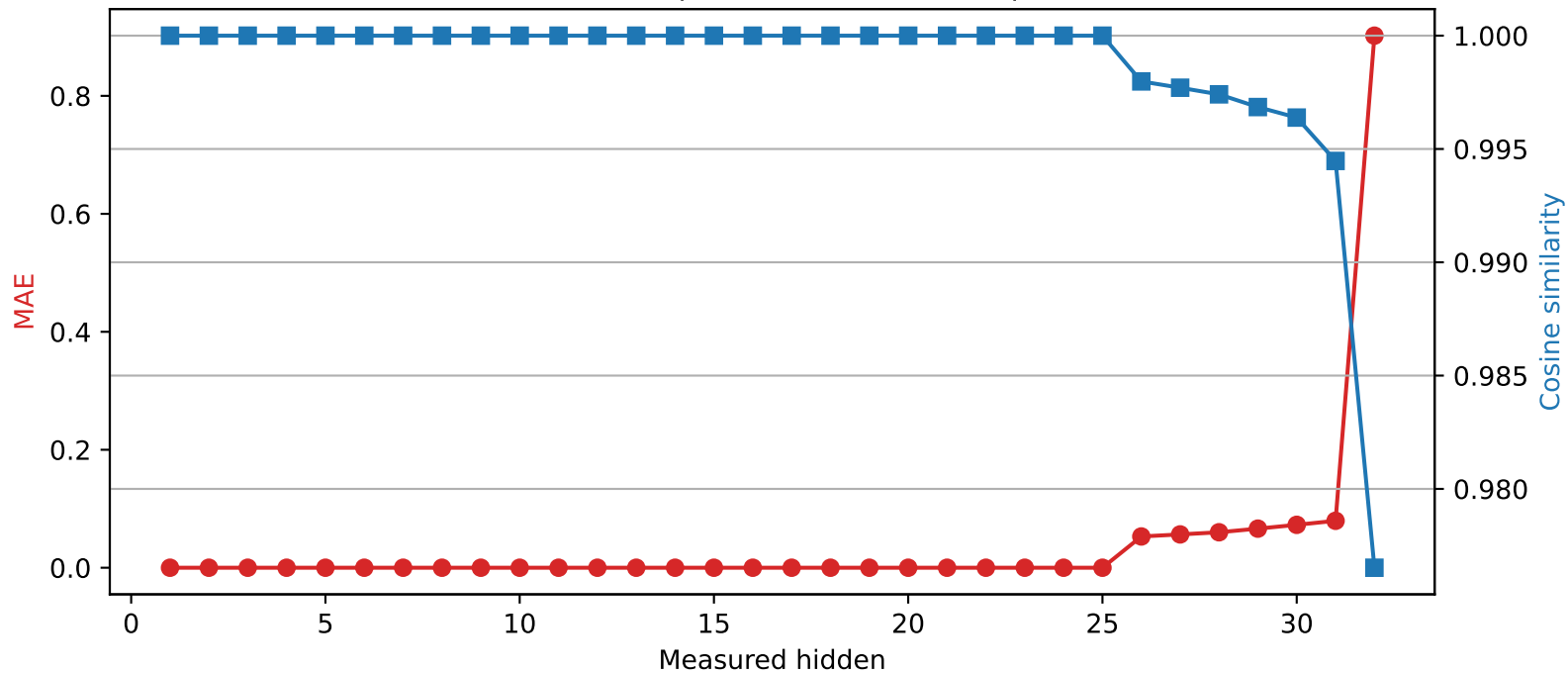
Mistral-7B-Instruct-v0.3 | Quantized layer 25 | float32 → int4
