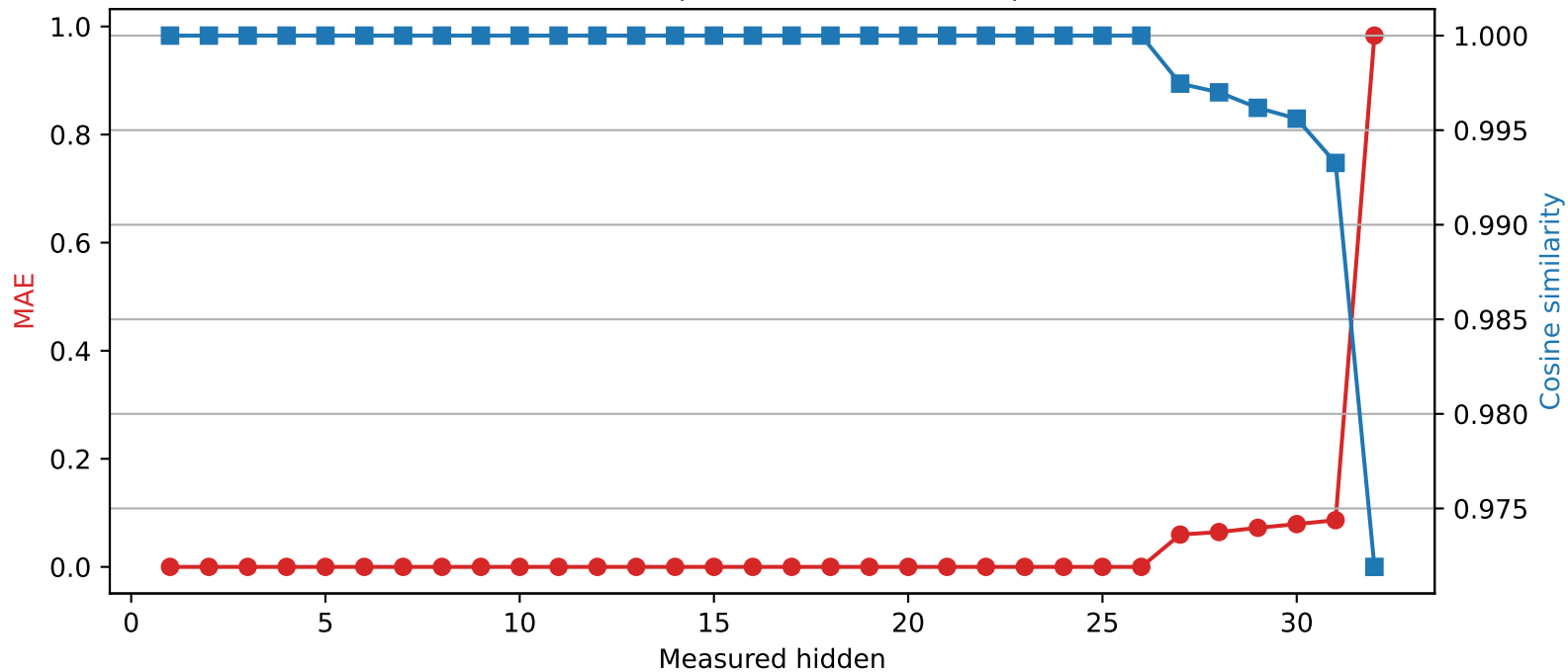
Mistral-7B-Instruct-v0.3 | Quantized layer 26 | float32 → int4
