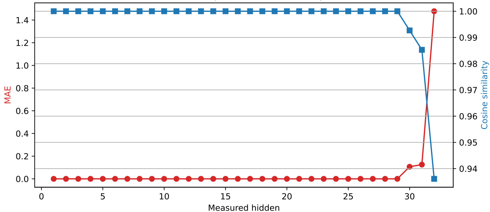
Mistral-7B-Instruct-v0.3 | Quantized layer 29 | float32 \rightarrow int4
