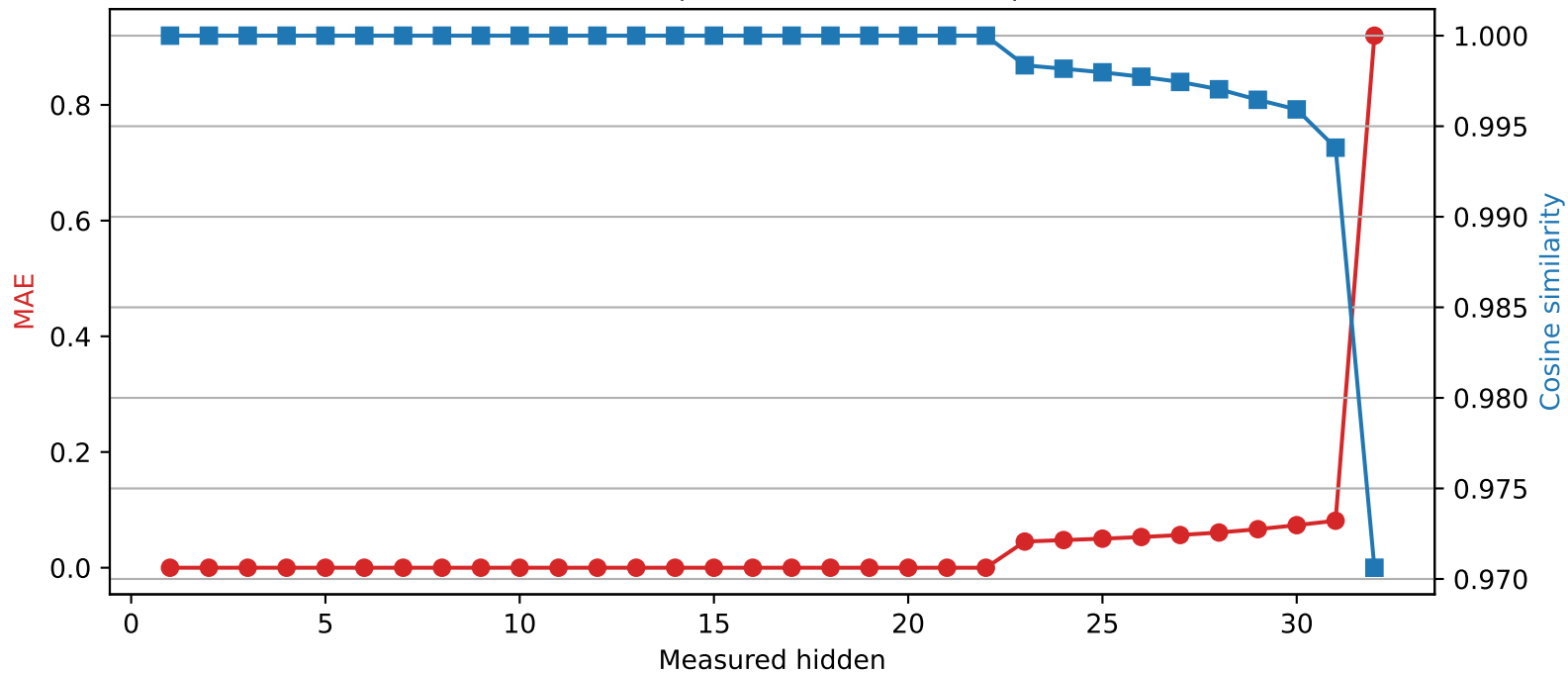
Mistral-7B-Instruct-v0.3 | Quantized layer 22 | float32 → int4
