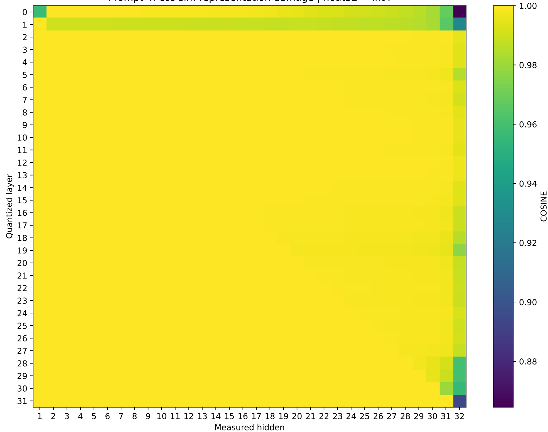
Mistral-7B-Instruct-v0.3 Prompt 4: cos sim representation damage | float32 → int4
