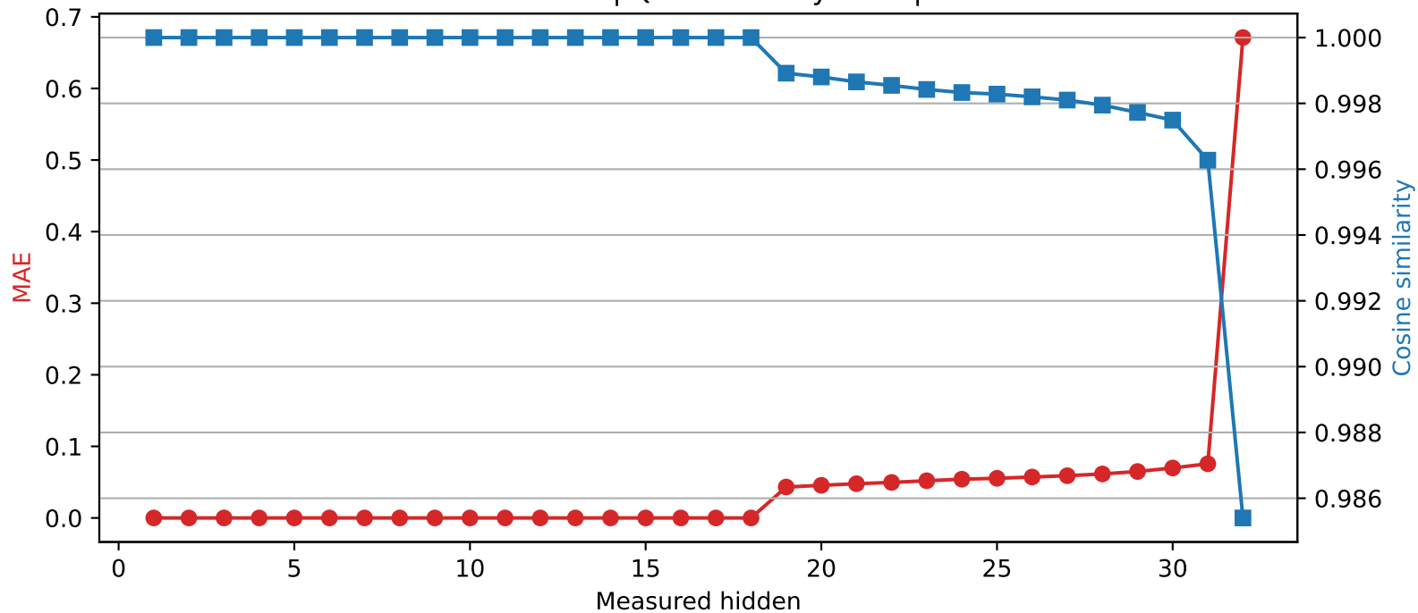
Mistral-7B-Instruct-v0.3 | Quantized layer 18 | float32 → int4
