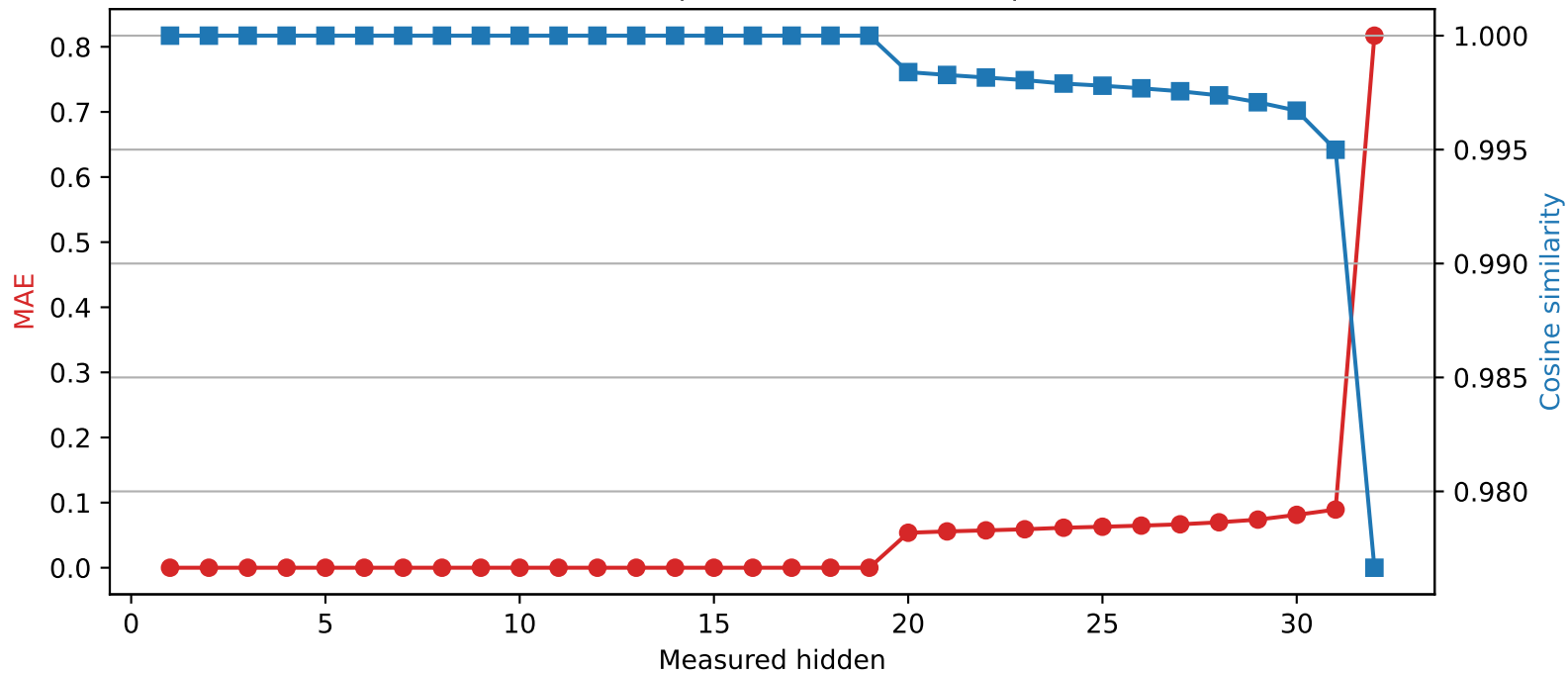
Mistral-7B-Instruct-v0.3 | Quantized layer 19 | float32 \rightarrow int4
