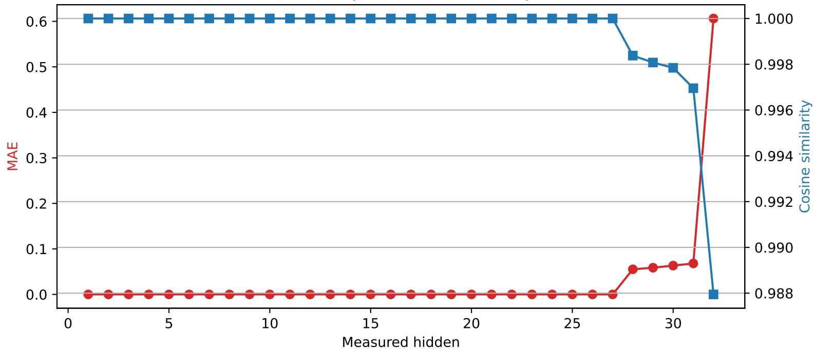
Mistral-7B-Instruct-v0.3 | Quantized layer 27 | float32 → int4
