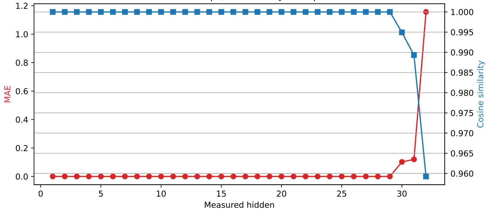
Mistral-7B-Instruct-v0.3 | Quantized layer 29 | float32 → int4
