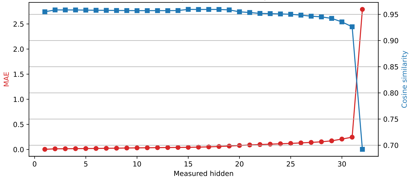
Mistral-7B-Instruct-v0.3 | Quantized layer 0 | float64 → int4
