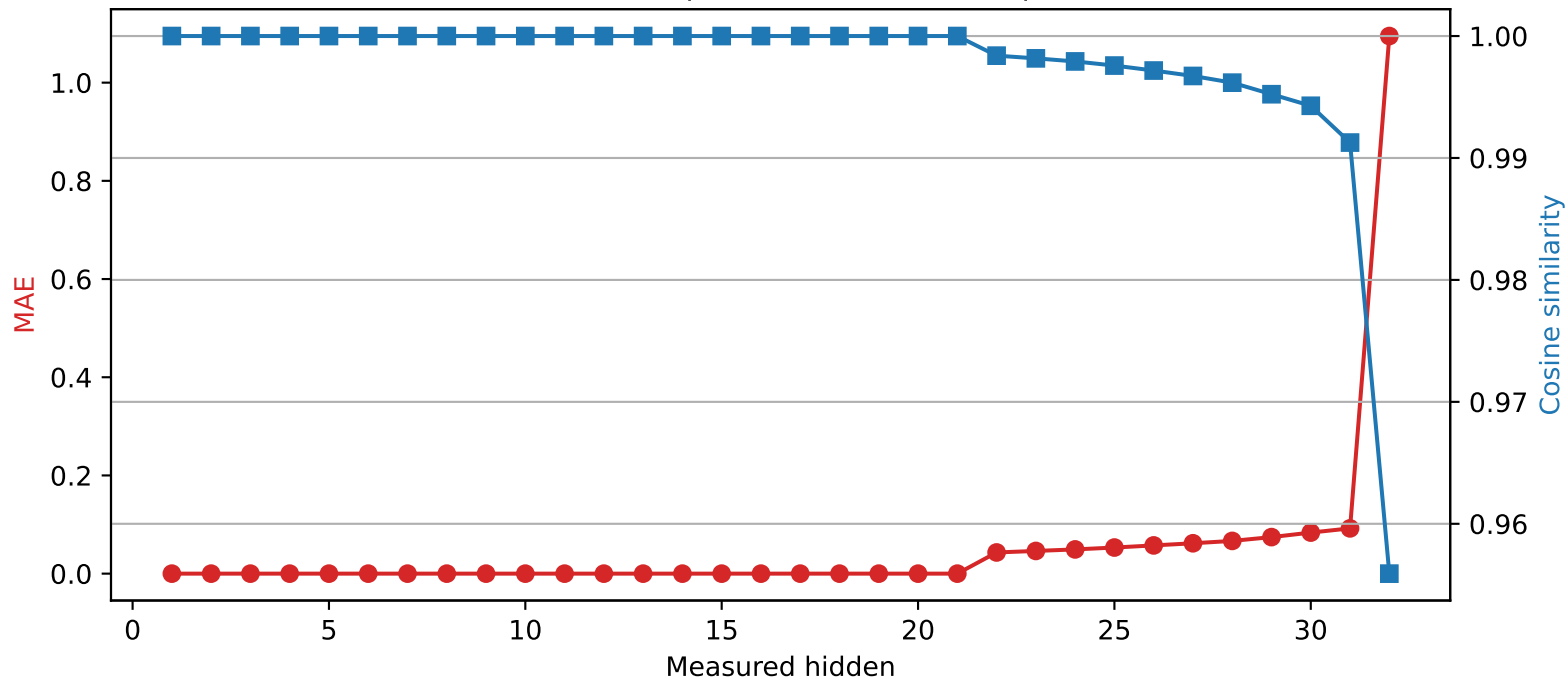
Mistral-7B-Instruct-v0.3 | Quantized layer 21 | float64 → int4
