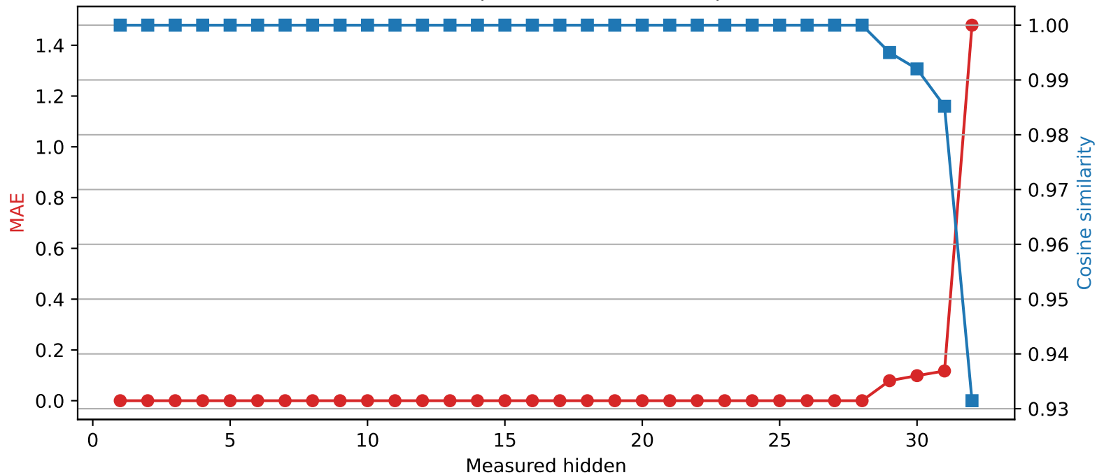
Mistral-7B-Instruct-v0.3 | Quantized layer 28 | float64 → int4
