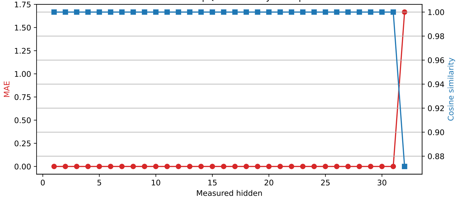
Mistral-7B-Instruct-v0.3 | Quantized layer 31 | float64 → int4
