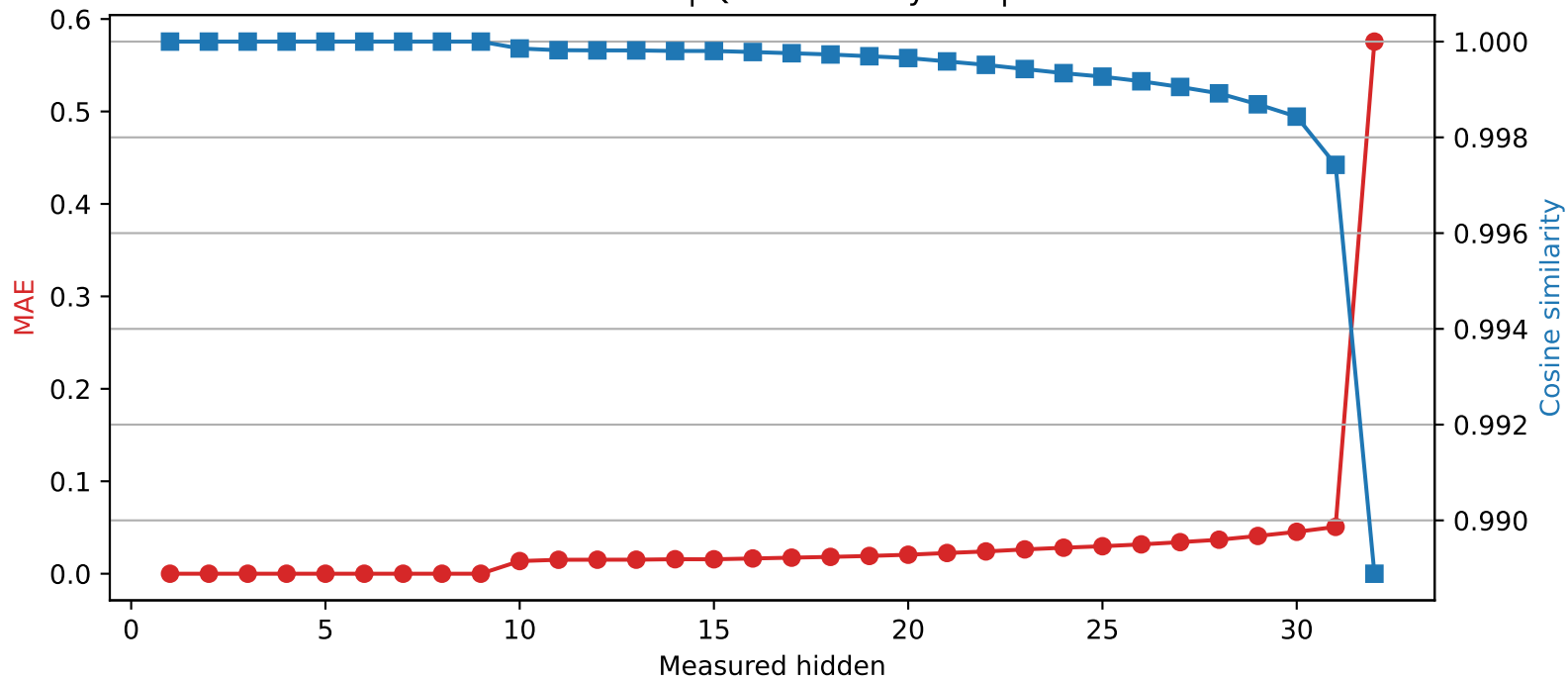
Mistral-7B-Instruct-v0.3 | Quantized layer 9 | float64 → int4
