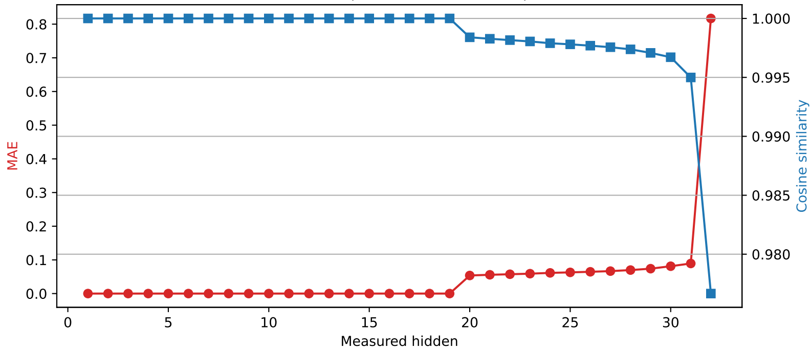
Mistral-7B-Instruct-v0.3 | Quantized layer 19 | float64 → int4
