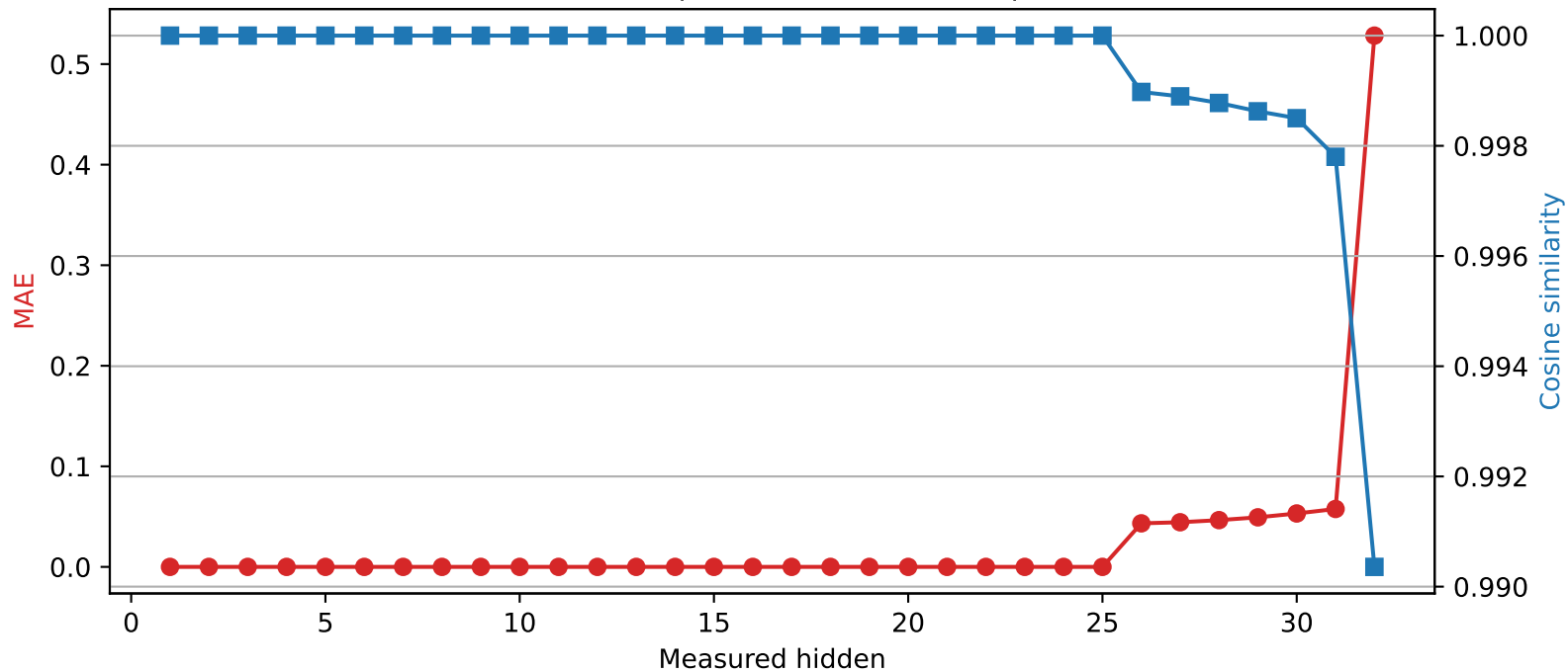
Mistral-7B-Instruct-v0.3 | Quantized layer 25 | float64 → int4
