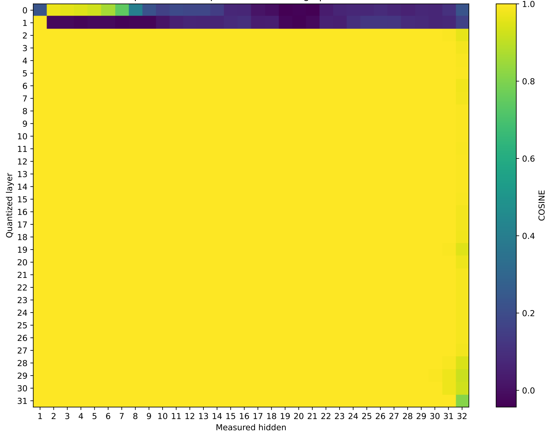
Mistral-7B-Instruct-v0.3 Prompt 0: cos sim representation damage | float16 \rightarrow int2
