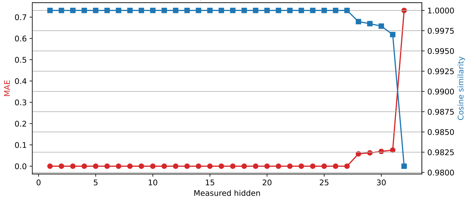
Mistral-7B-Instruct-v0.3 | Quantized layer 27 | float16 → int2
