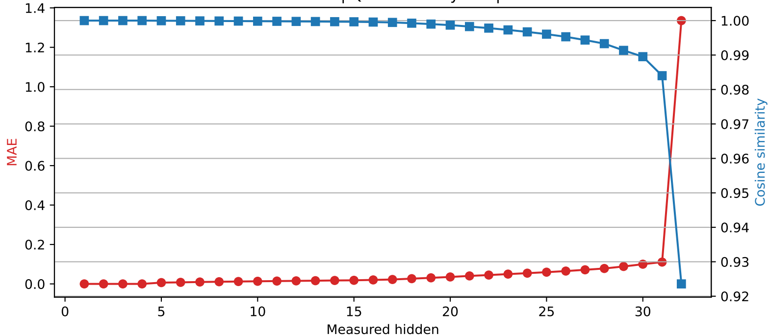
Mistral-7B-Instruct-v0.3 | Quantized layer 4 | float16 → int2
