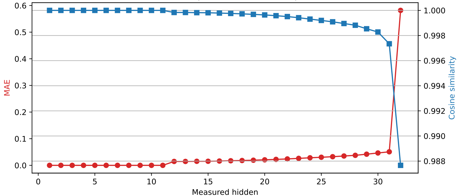
Mistral-7B-Instruct-v0.3 | Quantized layer 11 | float16 → int2
