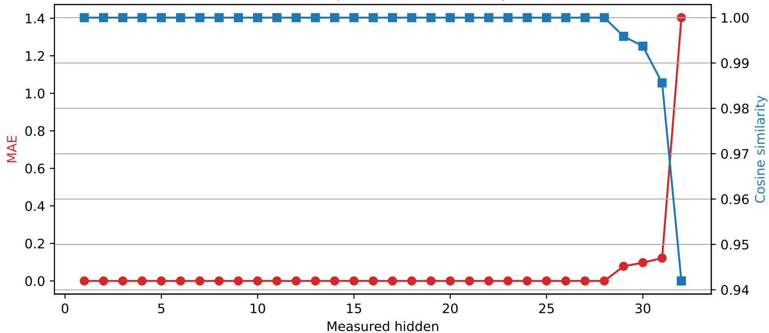
Mistral-7B-Instruct-v0.3 | Quantized layer 28 | float16 → int2
