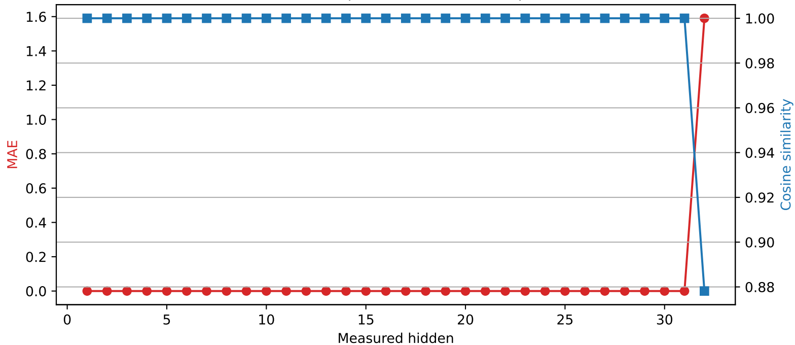
Mistral-7B-Instruct-v0.3 | Quantized layer 31 | float16 → int2
