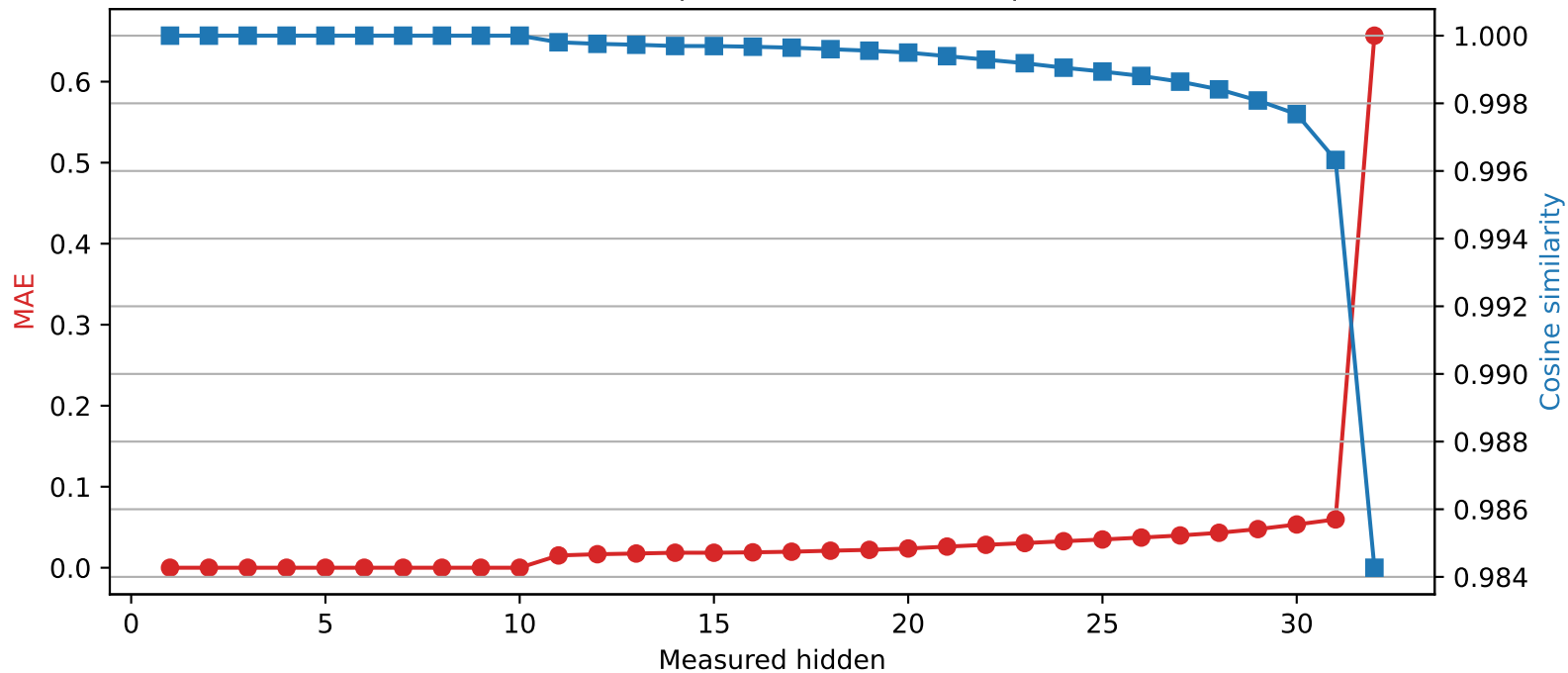
Mistral-7B-Instruct-v0.3 | Quantized layer 10 | float16 → int2
