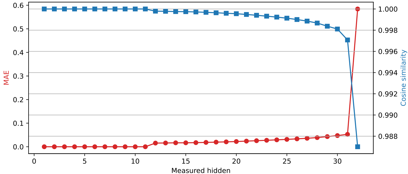
Mistral-7B-Instruct-v0.3 | Quantized layer 11 | float16 \rightarrow int2
