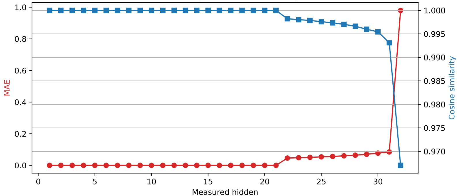
Mistral-7B-Instruct-v0.3 | Quantized layer 21 | float16 → int2
