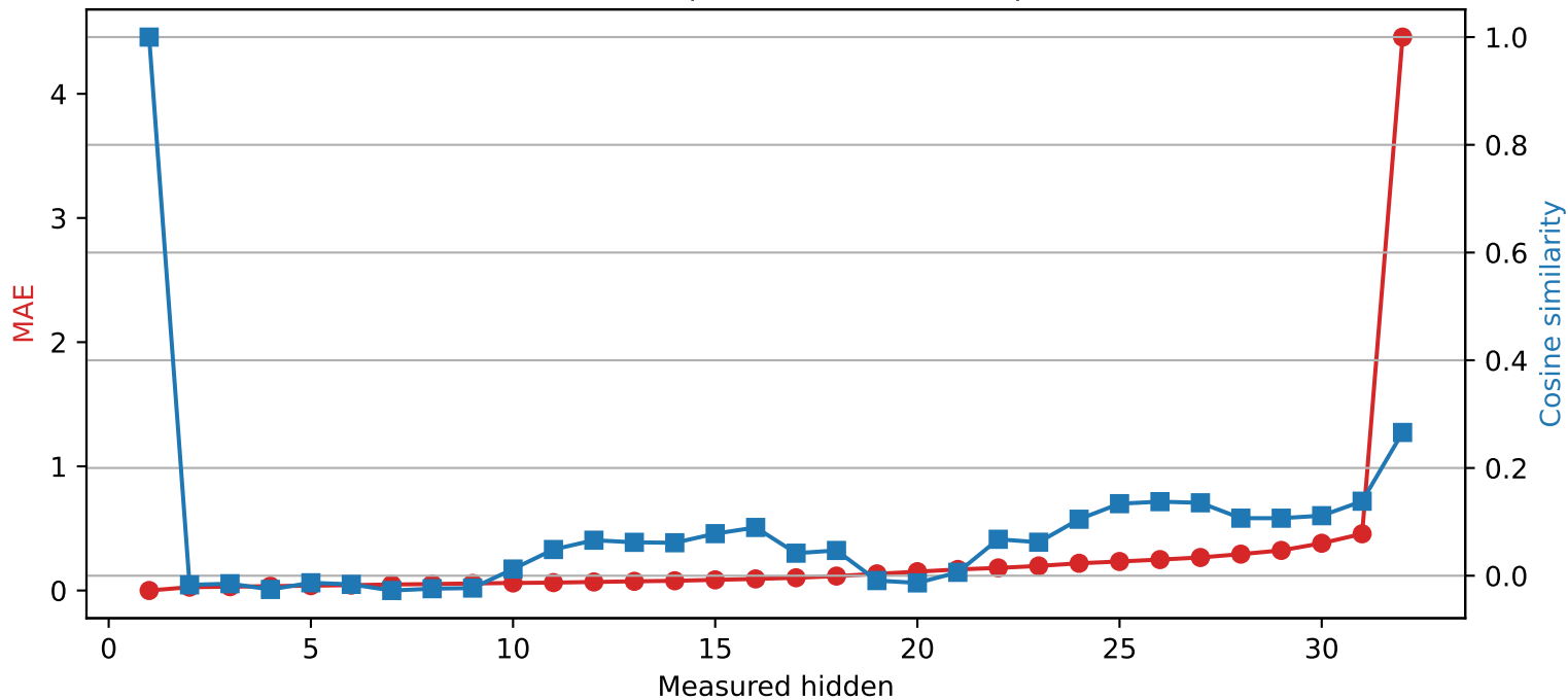
Mistral-7B-Instruct-v0.3 | Quantized layer 1 | float16 \rightarrow int2
