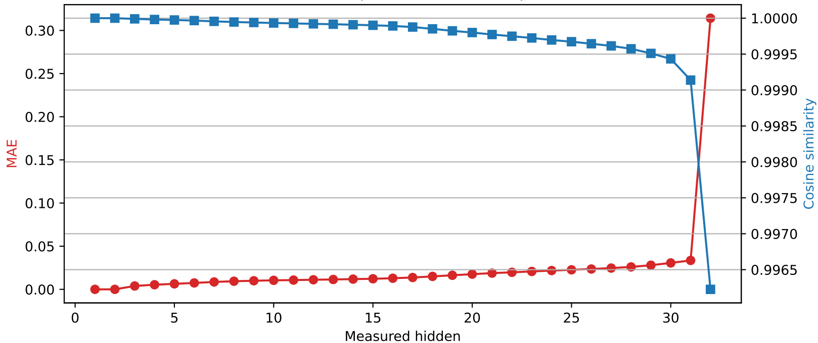
Mistral-7B-Instruct-v0.3 | Quantized layer 2 | float16 → int2
