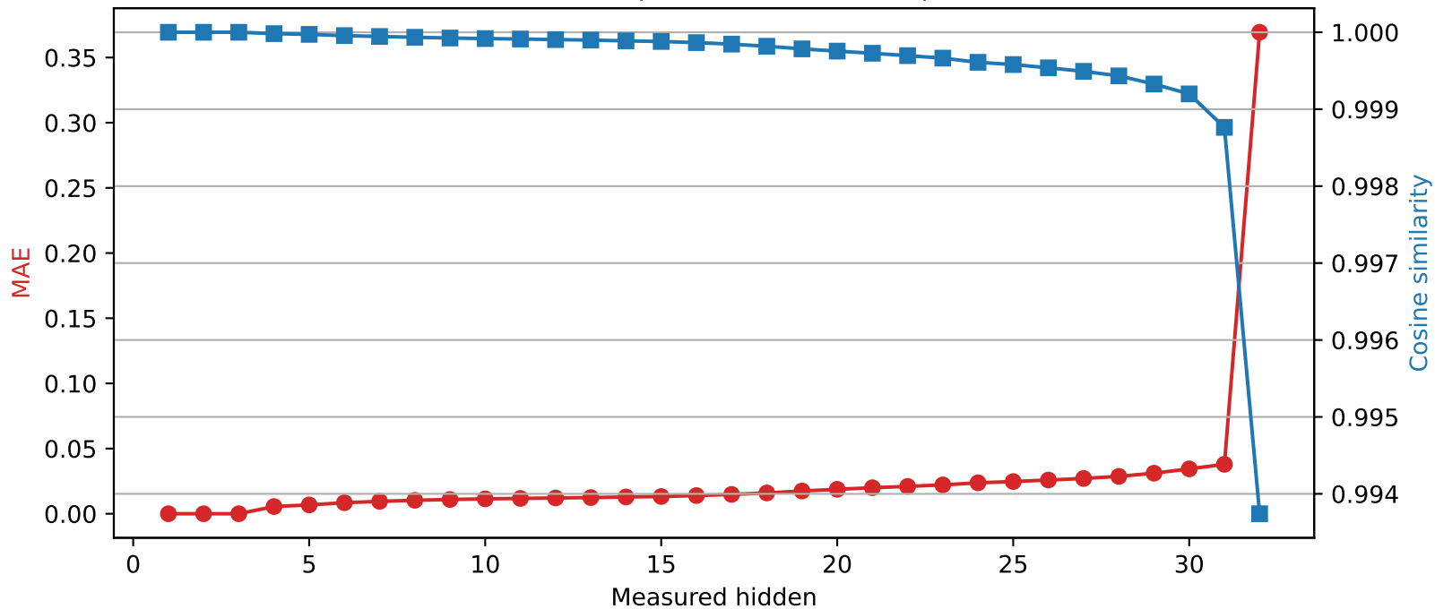
Mistral-7B-Instruct-v0.3 | Quantized layer 3 | float16 \rightarrow int2
