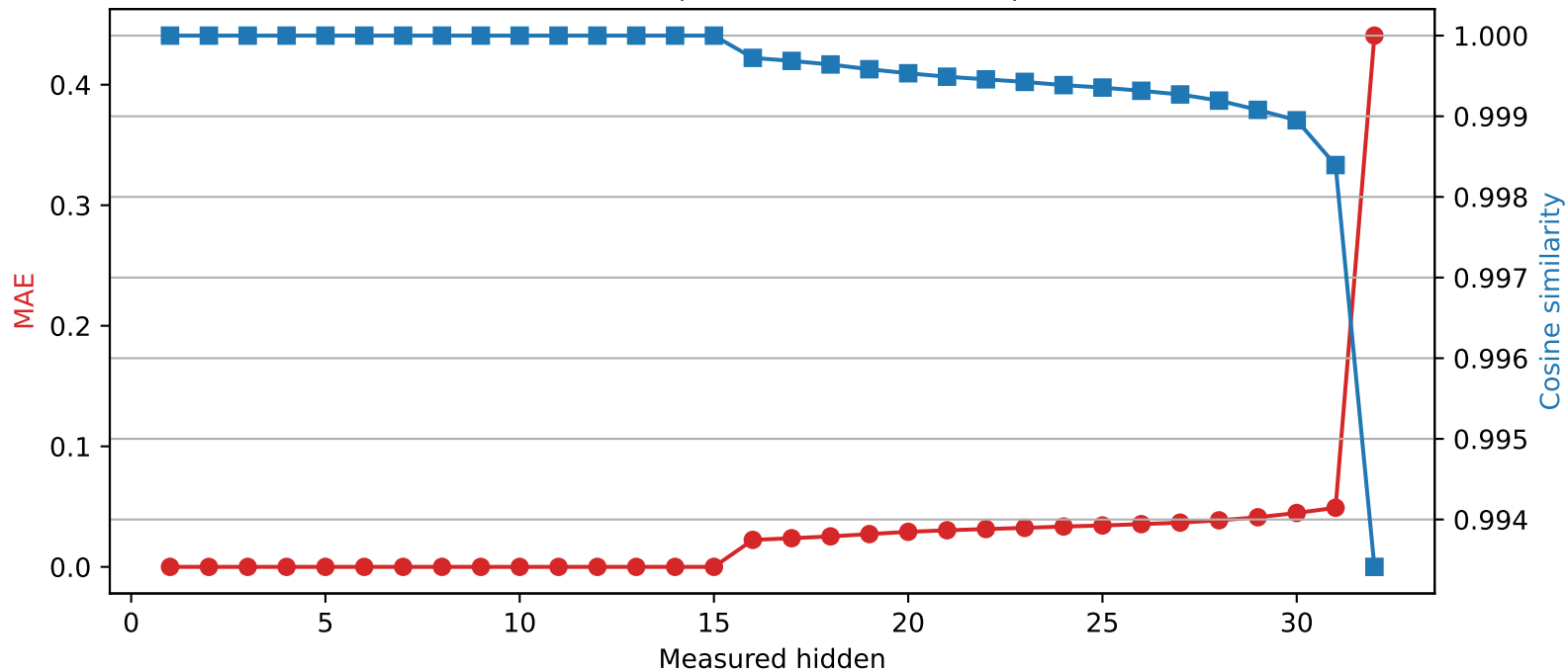
Mistral-7B-Instruct-v0.3 | Quantized layer 15 | float16 \rightarrow int2
