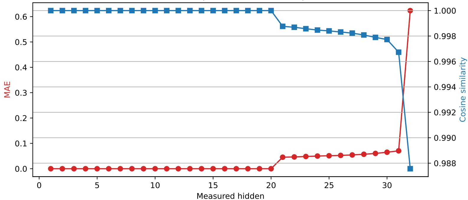
Mistral-7B-Instruct-v0.3 | Quantized layer 20 | float16 → int2
