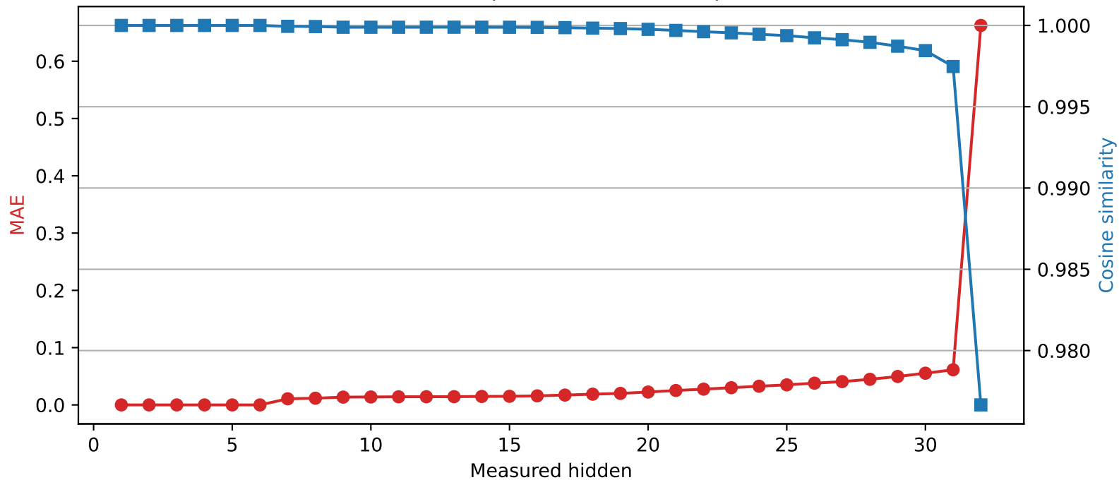
Mistral-7B-Instruct-v0.3 | Quantized layer 6 | float32 → int2
