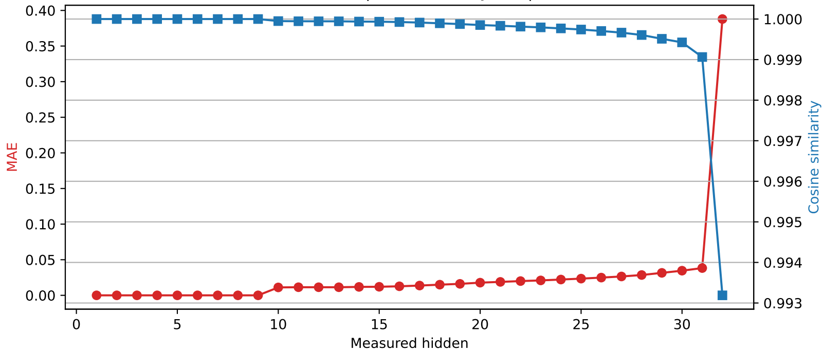
Mistral-7B-Instruct-v0.3 | Quantized layer 9 | float32 → int2
