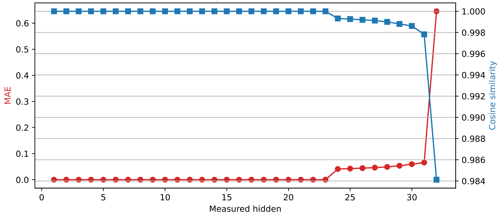
Mistral-7B-Instruct-v0.3 | Quantized layer 23 | float32 → int2
