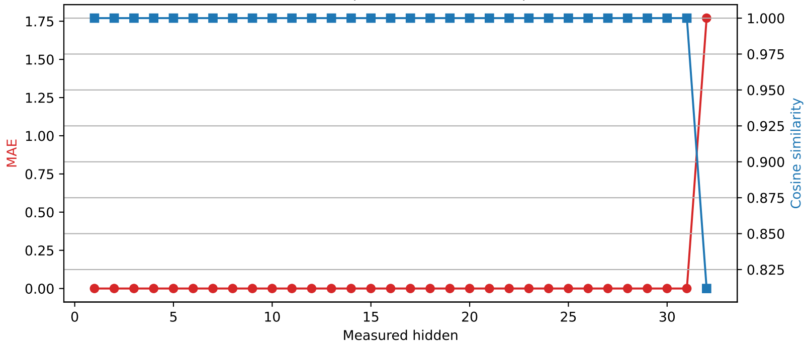
Mistral-7B-Instruct-v0.3 | Quantized layer 31 | float32 → int2
