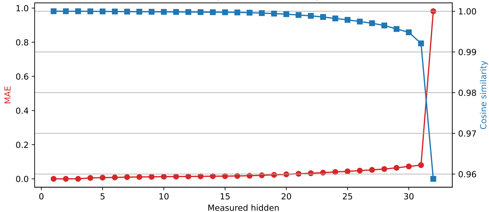
Mistral-7B-Instruct-v0.3 | Quantized layer 3 | float32 → int2
