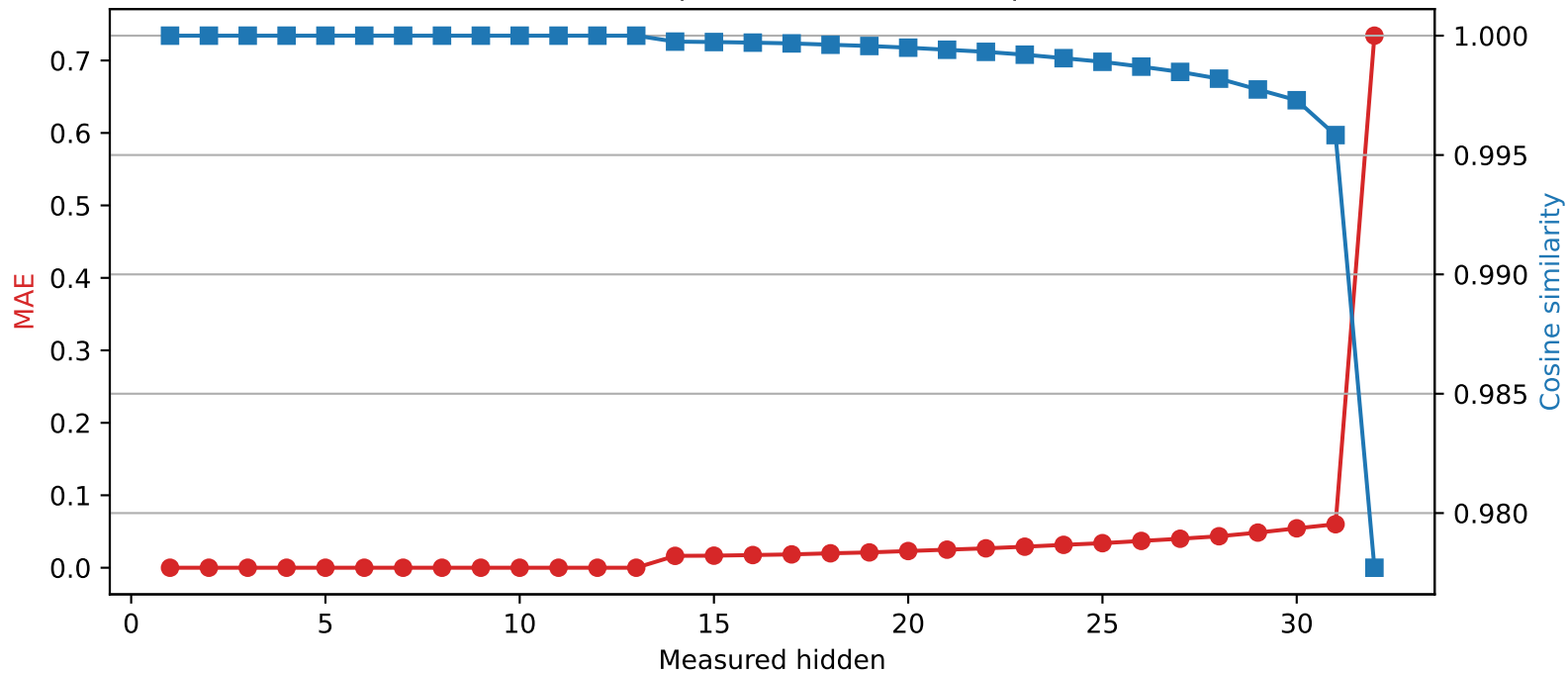
Mistral-7B-Instruct-v0.3 | Quantized layer 13 | float32 → int2
