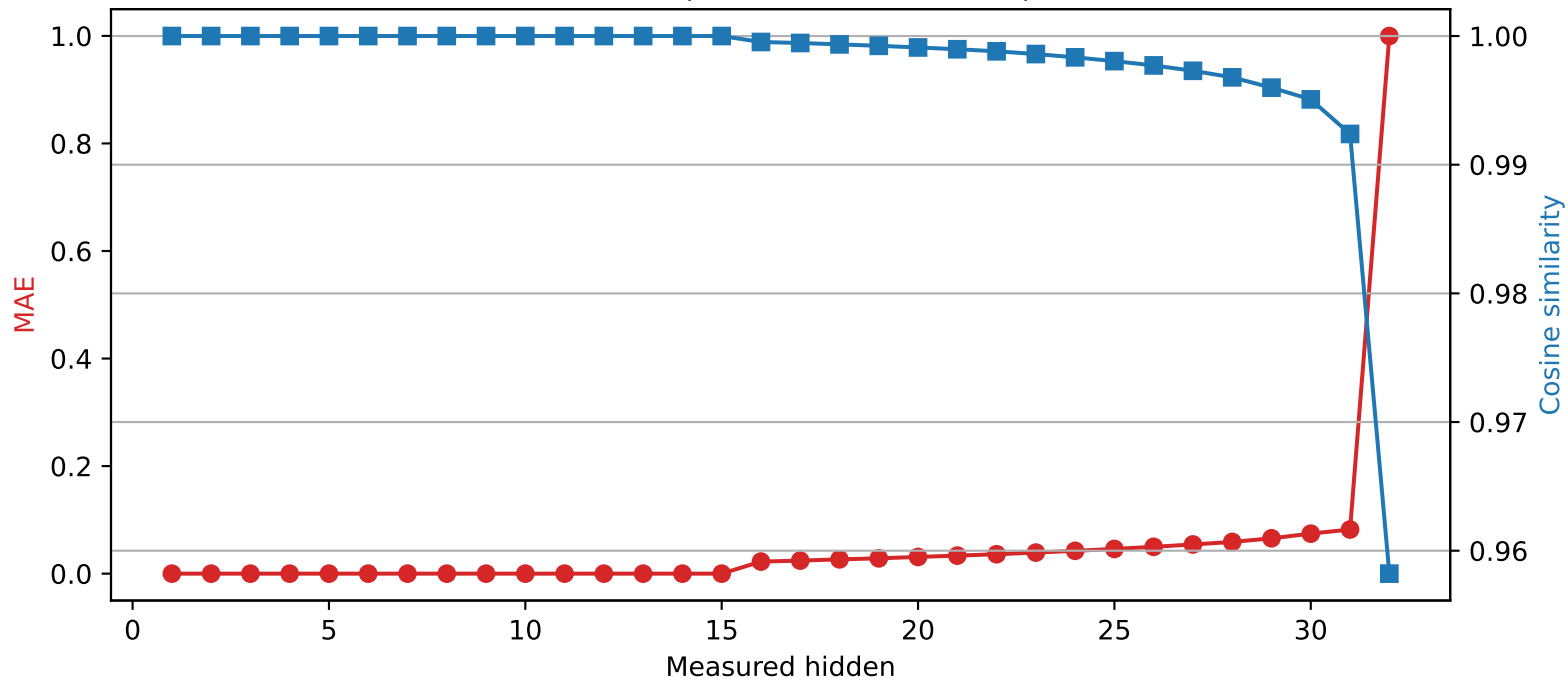
Mistral-7B-Instruct-v0.3 | Quantized layer 15 | float32 → int2
