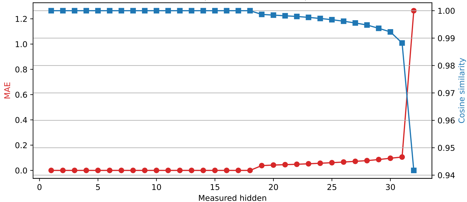
Mistral-7B-Instruct-v0.3 | Quantized layer 18 | float32 → int2
